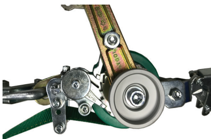
NEL-1500 MECHANISM
