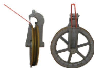
Urethane Lined with Helicopter Arm
