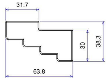
STEPPED BLOCK DIMENSIONS
