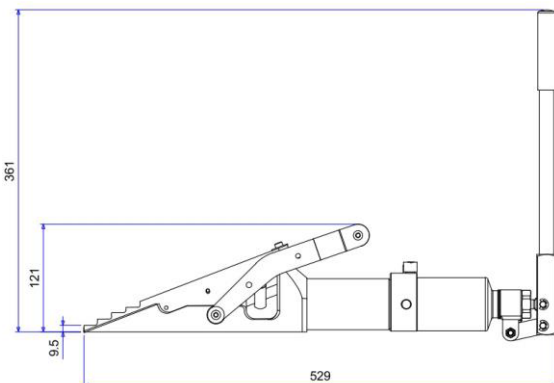
TOOL DIMENSIONS - CLOSED
