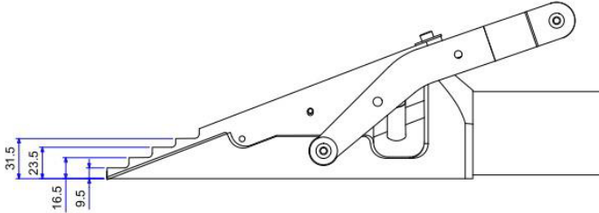
SAFETY BLOCK DIMENSIONS
