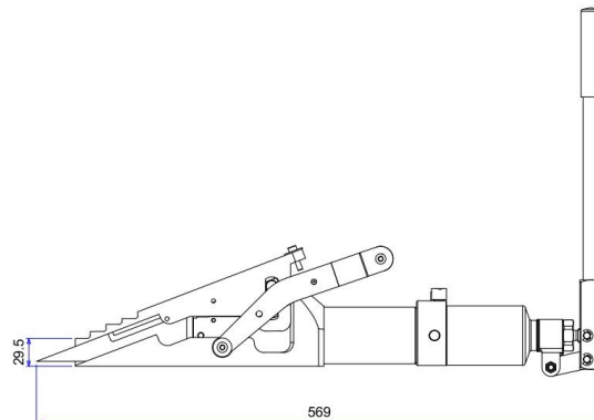
TOOL DIMENSIONS - OPEN
